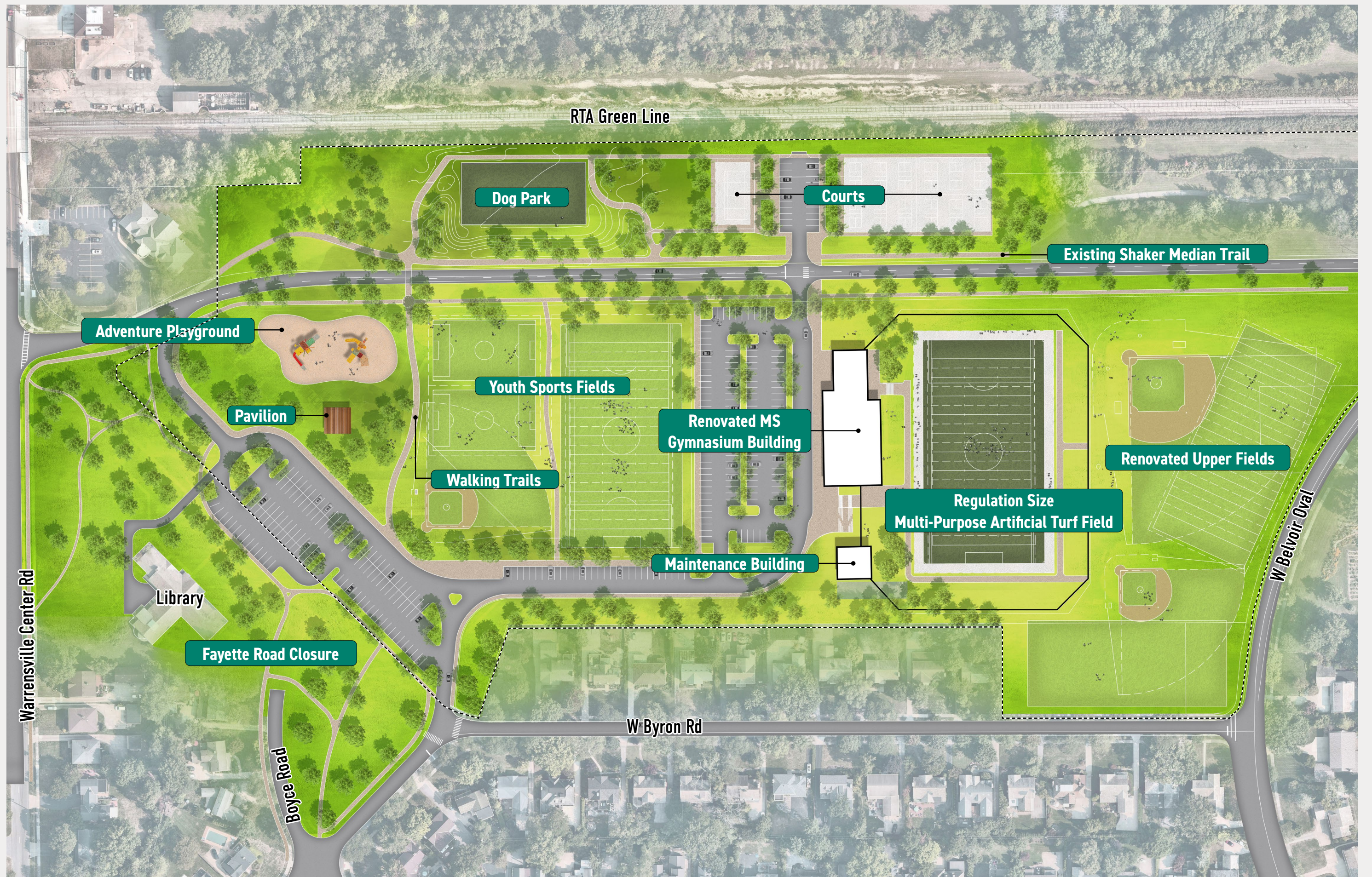
Shaker Heights Middle School Concept Plan 1
